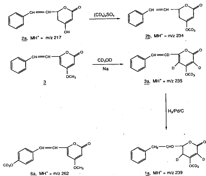
Scheme I—Chemical structures of the deuterated internal standards prepared for the GC-MS assay of dihydrokawain, kawain, desmethoxyyangonin, and yangonin (D = [ 2 H]). Protonated molecular ions [MH] + were recorded using methane CI-mass spectrometry.
